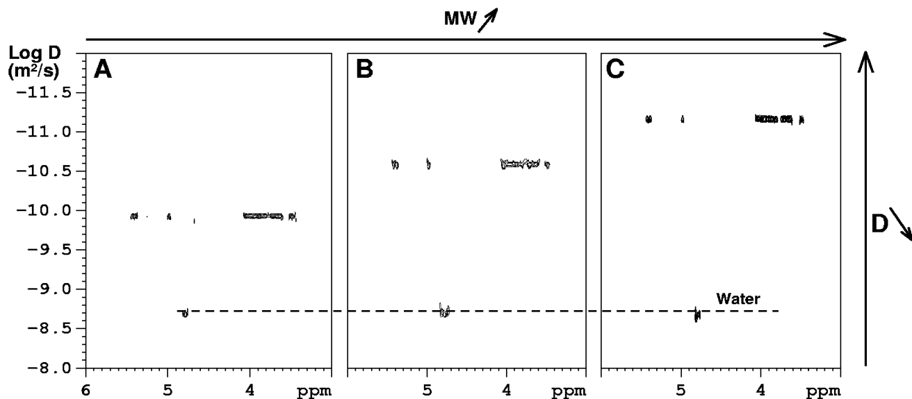
Figure 1. 2D DOSY spectra recorded in D 2 O at 300 K of three pullulan fractions with different molecular weights: M_W = 5.8 kDa (1a), M_W = 100 kDa (1b), and M_W = 853 kDa (1c).
